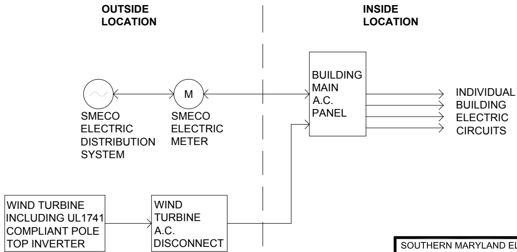
TYPICAL WIND TURBINE INTERCONNECTION CONFIGURATION
